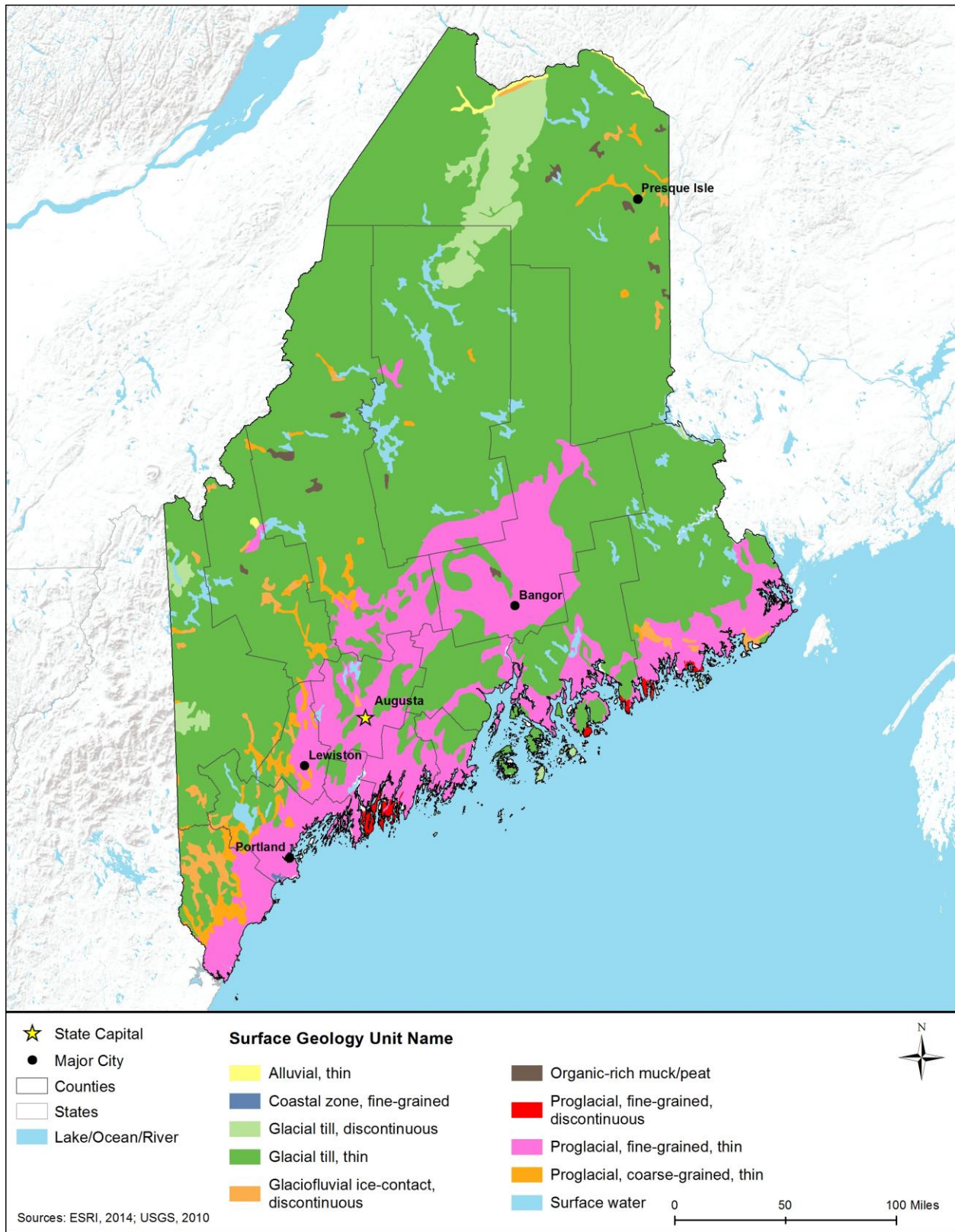
Figure 6.1.3-2: Generalized Surface Geology for Maine
